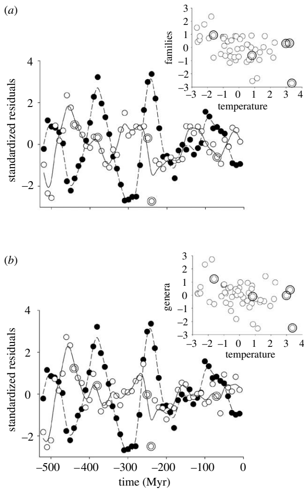
Figure 1. Taxonomic diversity against temperature. Time series of temperature and (a) standing diversity (number of families) using the maximum dating assumption and (b) standing diversity of boundary-crossing marine animal genera. Diversity and temperature were transformed, detrended and mean standardized. Closed circles and dashed lines represent temperature ( ^{\circ}\text{C} ) and open circles and continuous lines diversity. Large double open symbols represent periods of mass extinction, defined as the five largest positive extinction residuals (see text, figure 3). Curves are fitted using a 25 d.f. spline. Insets show the negative association between diversity and temperature residuals across the time series.
